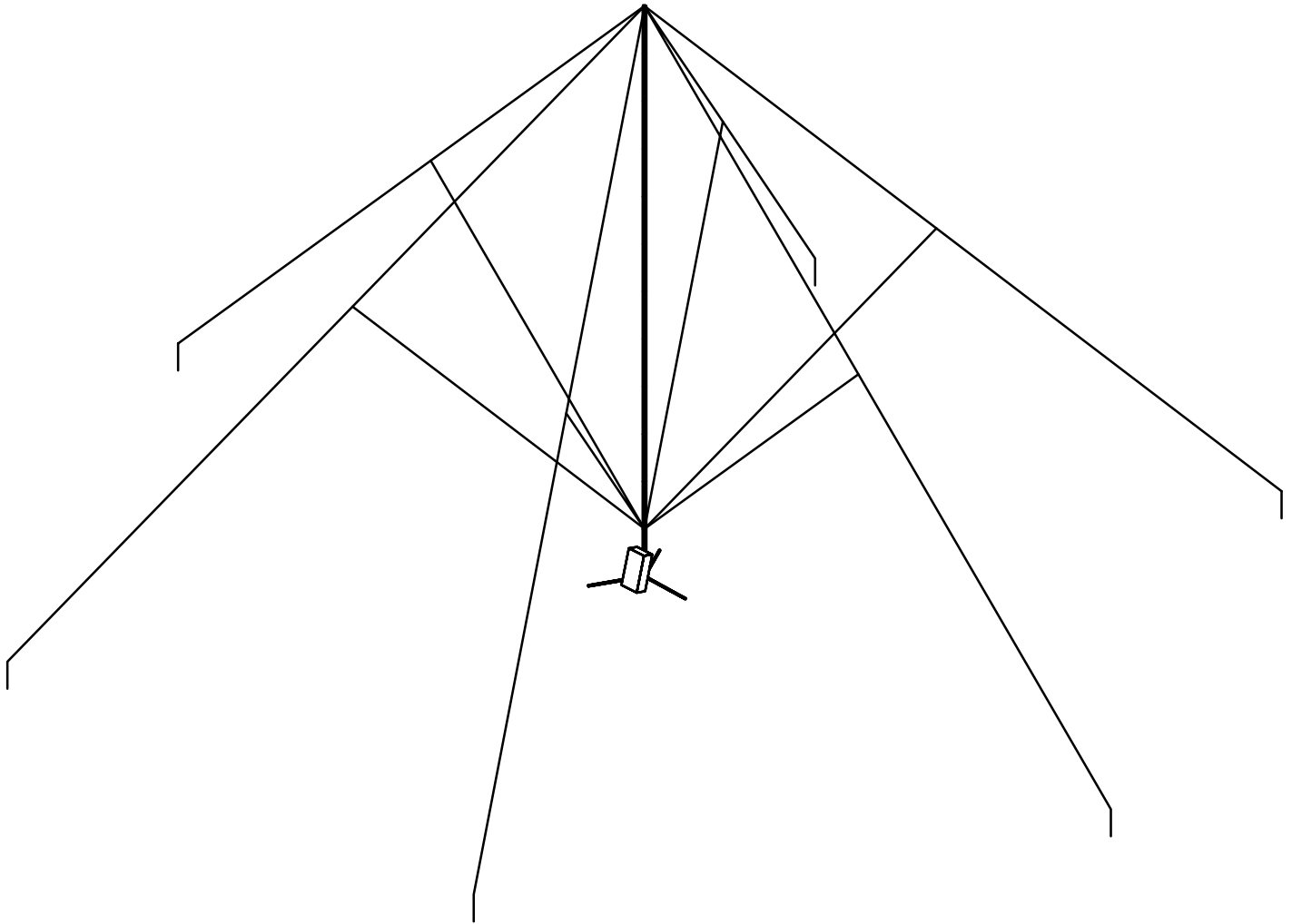
Diamond Portable Antenna (DPA) (Shown here to scale with SCARAB transmitter at base)
