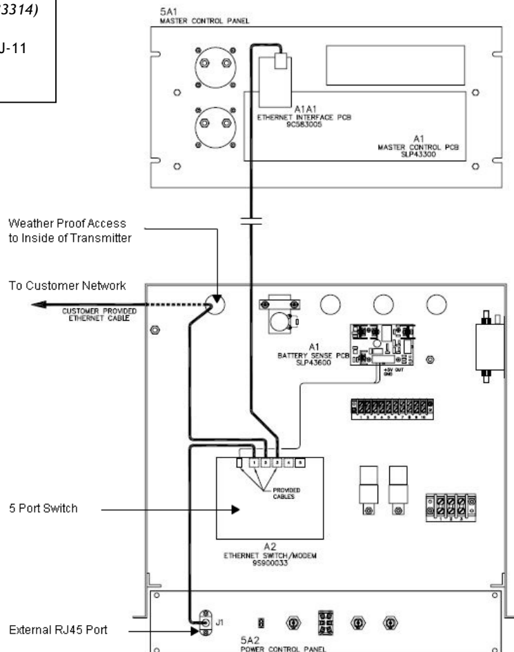
Internal View of 5 Port Switch
